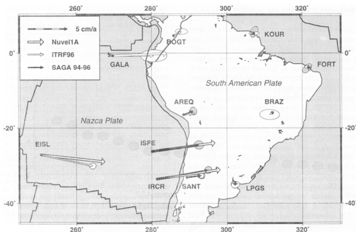
Figure 1: GPS data from four sites in the Nazca Plate (Easter Island, Galapagos, Robinson Crusoe and San Felix Islands) & from five sites in the stable core of the South American Plate used to calculate convergence rate [Angerman et. al., 1999] seismicity.
