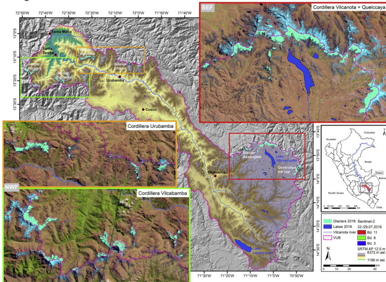
Figure 20: Overview of the Vilcanota-Urubamba-Vilcabamba basin (VUB) situated in Peru (rectangle in the small overview map) with main cities (red circles), prominent glaciers (turquoise triangles) and two principal reservoirs (Sibinacocha and Langui Loy). Glaciers belonging to the VUB (dashed pink delimitation) are highlighted as turquoise area. NWF=northwestern glacier fragment, SEF=southeastern glacier fragment. Reproduced from Drenkham et al., 2018.
