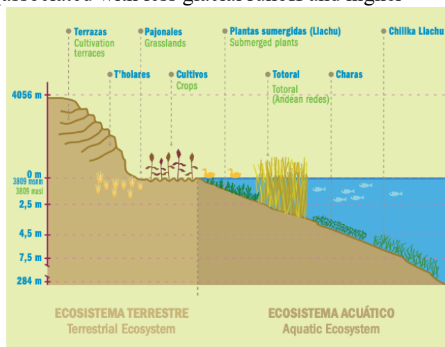
Figure 6: Illustration of aquatic and terrestrial agricultural and ecosystem zones in the Lake Titicaca basin (globalnature.org)
