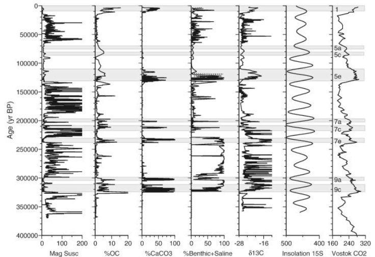
Figure 5: Multiproxy lake sediment record for the Titicaca basin showing glacial-interglacial cycles, with %organic carbon, %calcium carbonate, %Benthic+saline foraminifera, and δ13C increasing during interglacial periods (high Vostok CO 2 ), and magnetic susceptibility increasing during glacials (low Vostok CO 2 )(Fritz et al., 2012)
