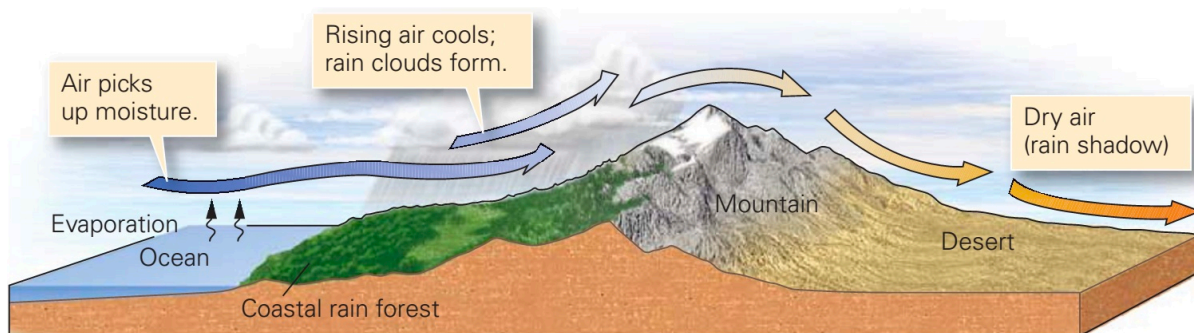
Figure 21 – Cartoon illustrating the formation of rain shadow deserts. From Marshak, 2015.
