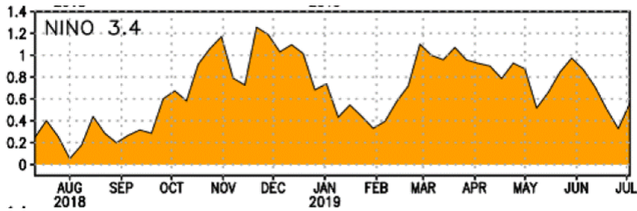
Figures 8 and 9— Top: SST anomalies ( ^{\circ} C) in the Nino 3.4 region in late 2018 and early 2019 Left: forecasted SST anomalies in the Nino 3.4 region (Climate Prediction Center)
