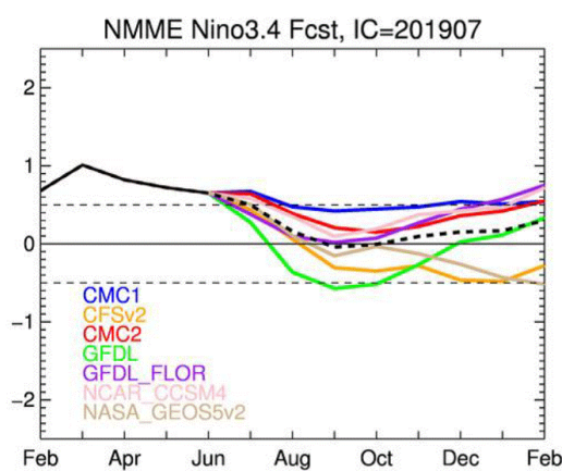
Figures 8 and 9— Top: SST anomalies ( ^{\circ} C) in the Nino 3.4 region in late 2018 and early 2019 Left: forecasted SST anomalies in the Nino 3.4 region (Climate Prediction Center)
