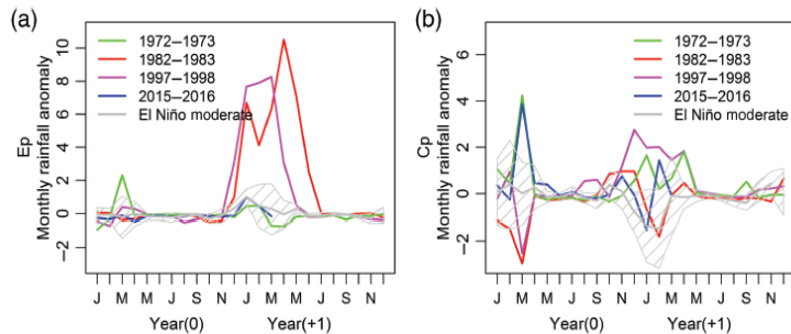
Figure 7—Top: Difference in spatial rainfall pattern during eastern Pacific (Ep) and central Pacific El Niño events. Bottom: Difference in temporal signature of eastern and central Pacific El Niño events (Sanabria et al., 2018)
