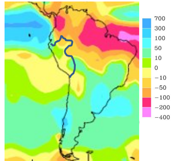
Figure 3—Precipitation anomaly (mm) during the average El Niño event (Dai and Wigley, 2000)
